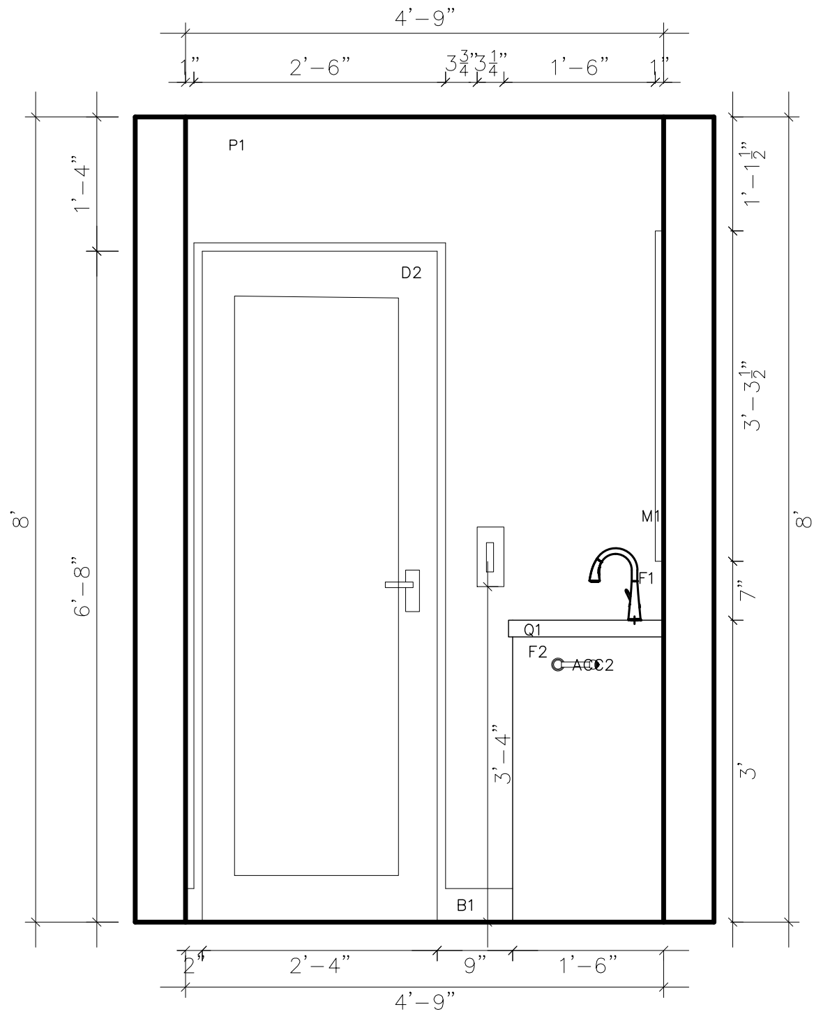
1 WEST ELEVATION 105 SCALE: 3/4" = 1'-0"
