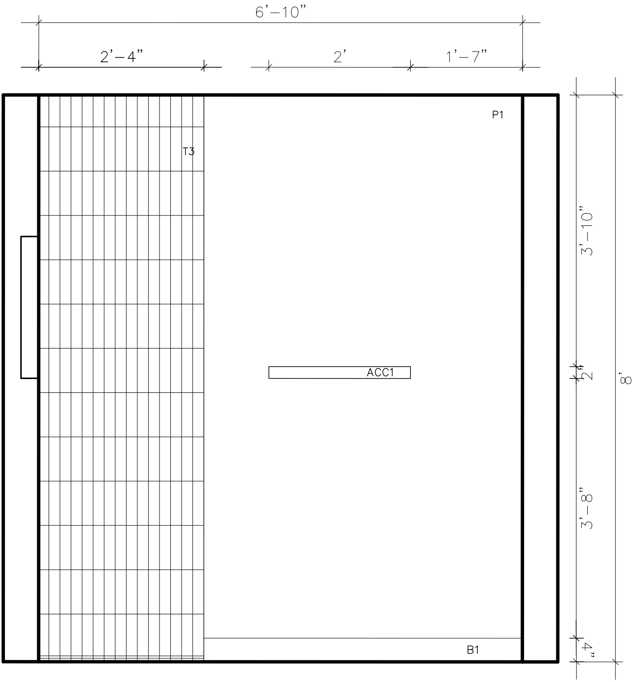
2 SOUTH ELEVATION 106 SCALE: 3/4" = 1'-0"
