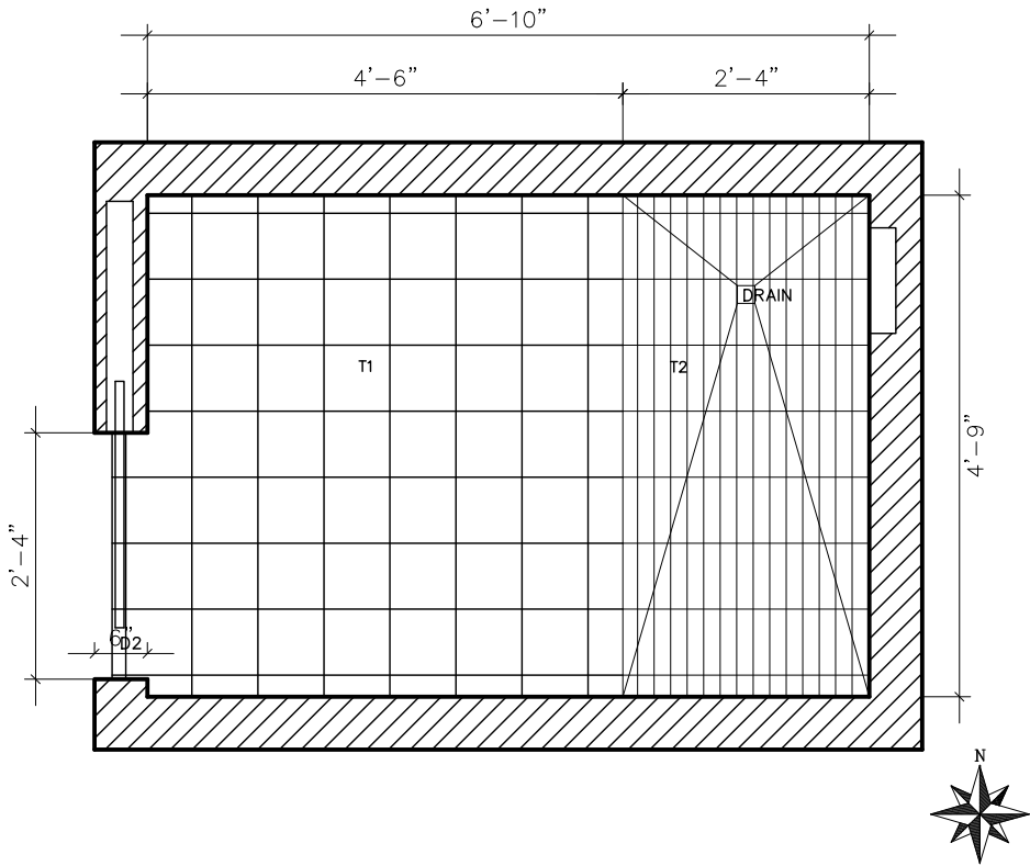
2 FLOOR FINISH PLAN 103 SCALE: 1/2" = 1'-0"
