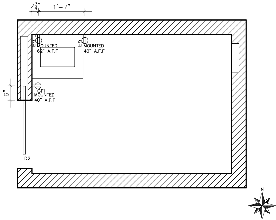
2 ELECTRICAL PLAN 102 SCALE: 1/2" = 1'-0"
