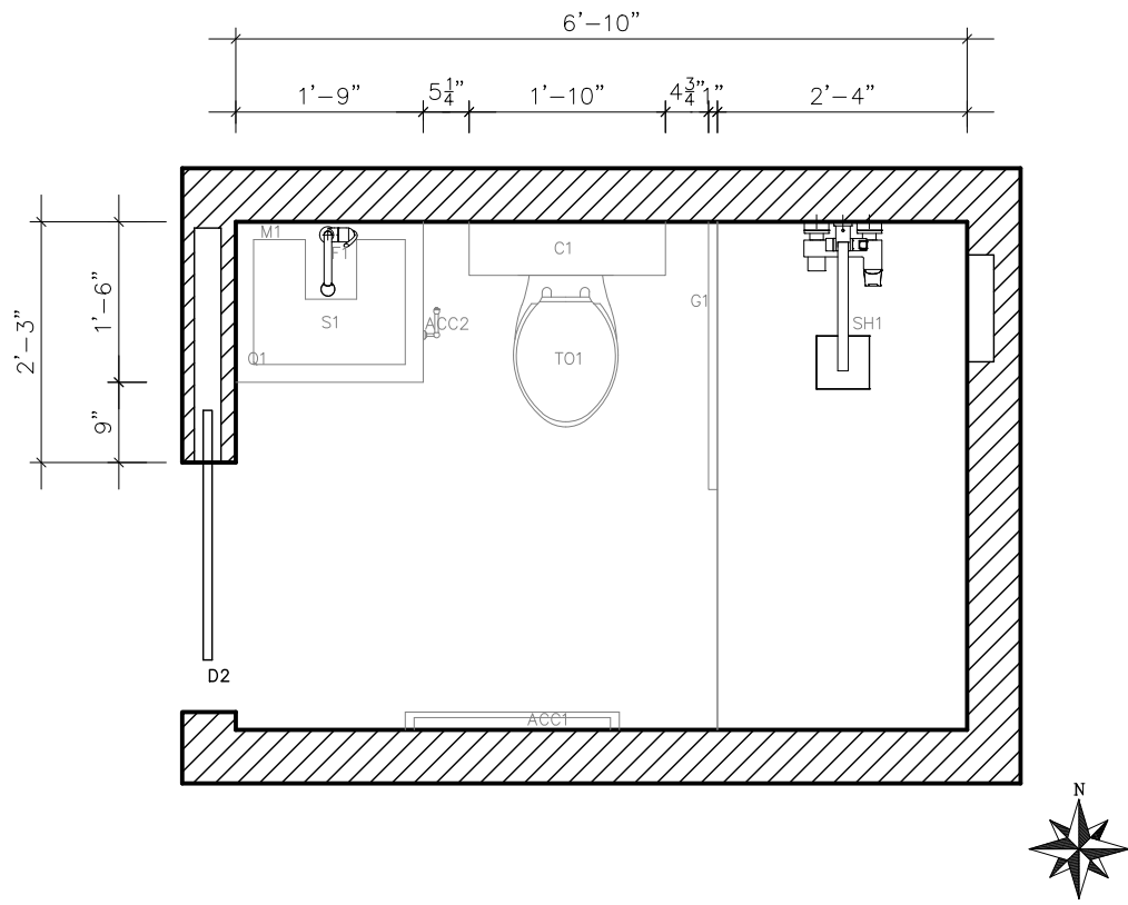
1 MILLWORK PLAN 104 SCALE: 1/2" = 1'-0"
