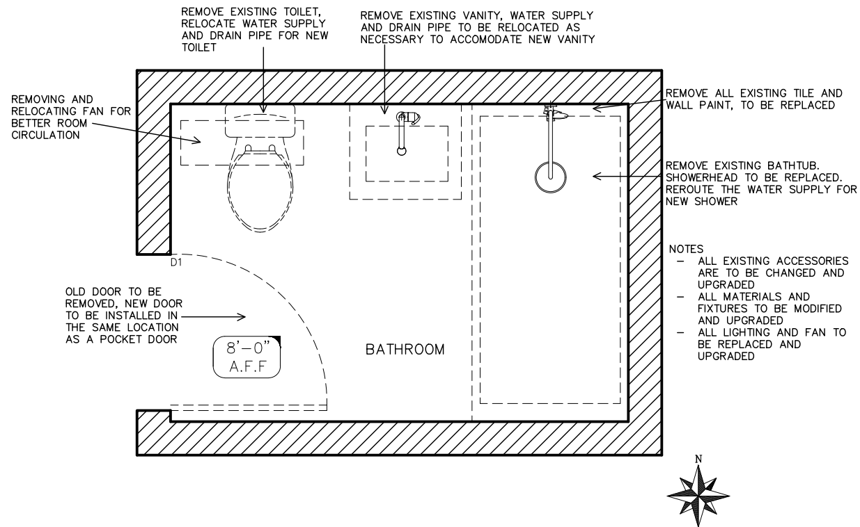
2 DEMOLITION PLAN 101 SCALE: 1/2" = 1'-0"
