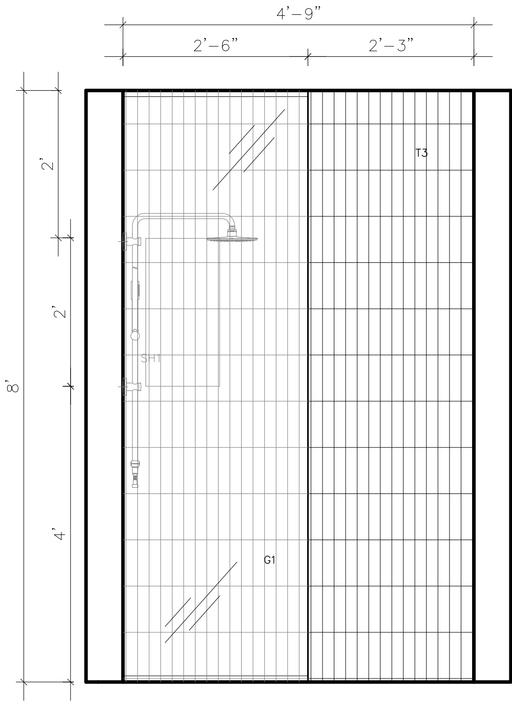
1 EAST ELEVATION 106 SCALE: 3/4" = 1'-0"
